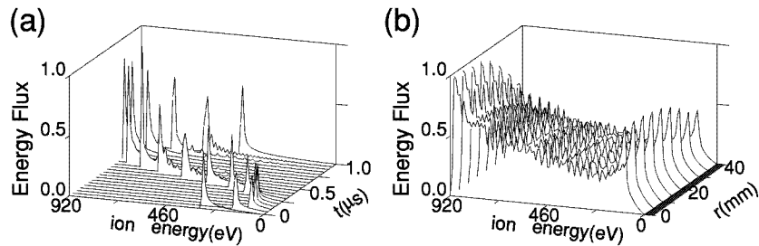
FIGURE 6. Ion energy distribution on the electrode as a function of radial distance in 1f-CCP driven at 100 MHz and 300 V at 50 mTorr in \text{CF}_4(5\%)/\text{Ar} .
